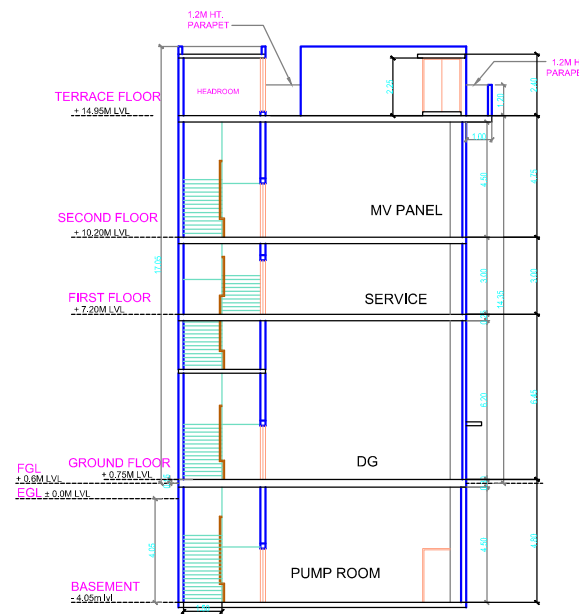
SECTION - Y1
