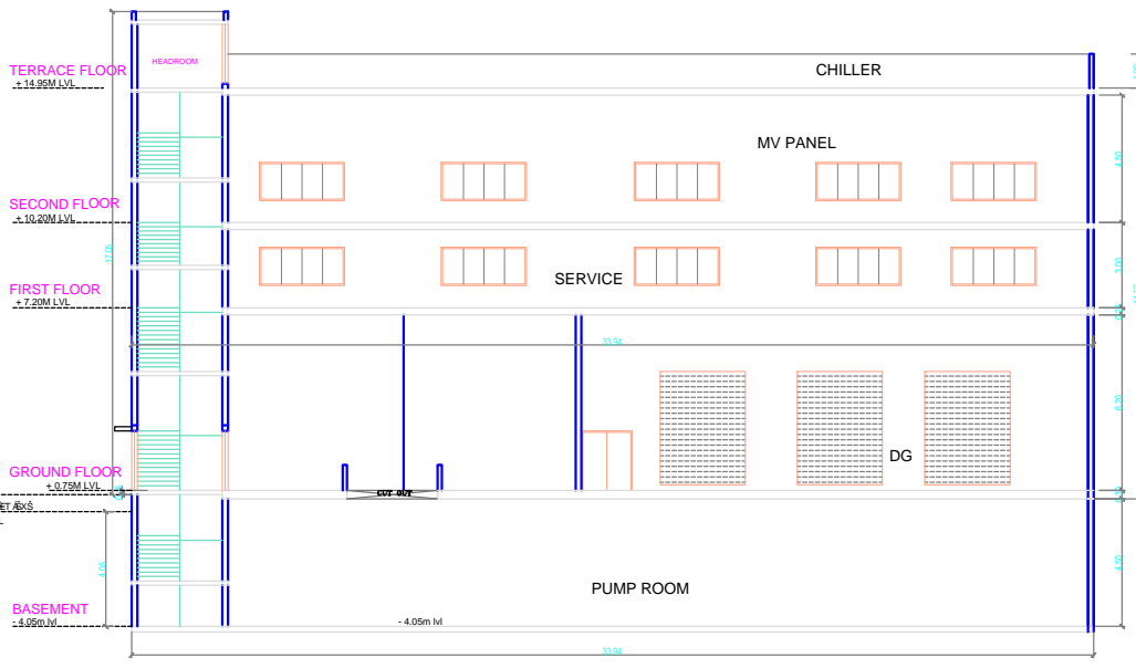
SECTION - X1
