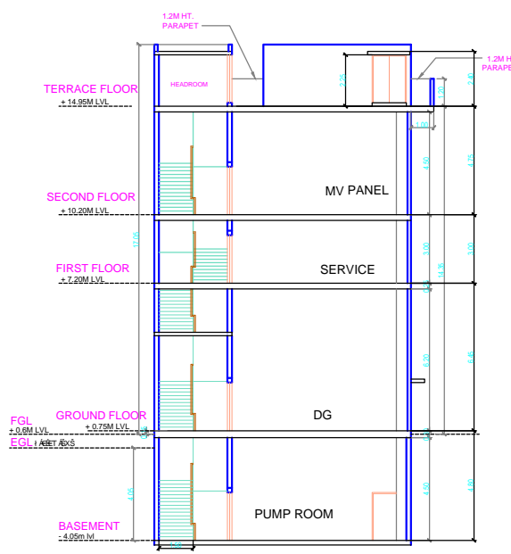
SECTION - Y1
