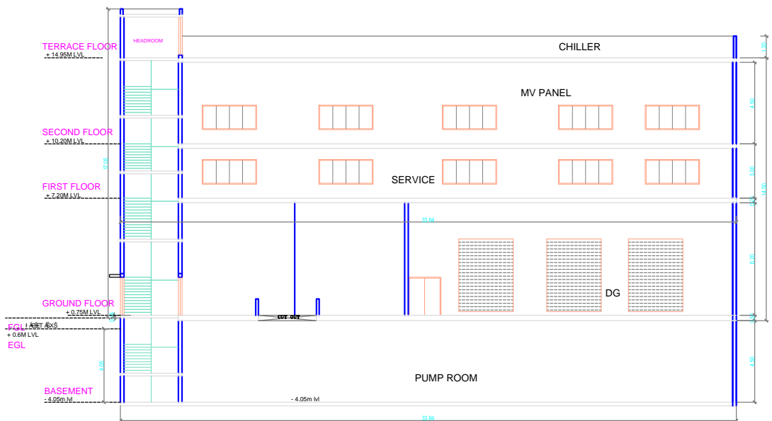
SECTION - X1
